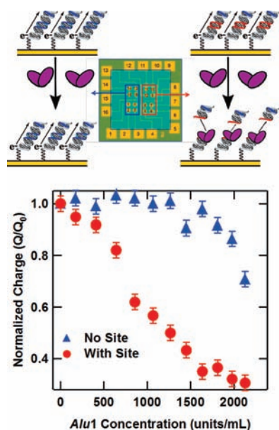
Figure 3. Restriction assay on the DME chip. (upper) Illustration of sequence-specific activity of the Alu1 restriction enzyme electrochemically monitored with a DME chip. (lower) Charge versus Alu1 concentration for a DME chip for DNA with (red) and without (blue) the Alu1 restriction site. In particular, the sequence of the DNA containing the restriction site was the well matched 17-mer 5'- T NB GC GTC TCA GCT GAA GT-3', where the italicized bases represent the restriction site and T NB is a thymine modified with a Nile Blue redox probe. The sequence absent this site but containing a three-base pseudosite was the well matched 17-mer 5'- T NB GC GTG CTT TAT ATC TC-3', with the pseudosite given in italics. Charge was obtained by integrating the cathodic Nile Blue CV peaks obtained at a 50 mV/s scan rate after equilibration of the Alu1 activity at each concentration.
