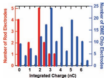
Figure 4. Histogram of the total charge from DNA monolayers from the electrodes of 9 DME chips (blue) and 15 rod electrodes (red). Both types of electrodes were coated with well matched DNA monolayers with the sequence 5'- T NB GC GTG CTT TAT ATC TC-3', where T NB is a Nile Blue modified thymine. The integrated charge was obtained by integrating the cathodic peak of the cyclic voltammogram taken at a 50 mV/s scan rate. For ease of comparison, integrated charges have been sorted according to the nearest half coulomb. Note that on average a much higher signal and fewer failures (signals <0.5 nC) are found for gold electrodes on DME chips.
