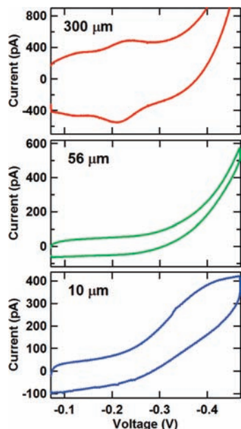
Figure 5. Average cyclic voltammetry (CV) signals from Nile Blue DNA-modified 300, 56, and 10 \mu\text{m} diameter electrodes prepared on the same chip. The electrodes were assembled with 17-mer DNA duplexes of the sequence 5'- T_{NB} GC GTC TCA GCT GAA GT-3' and the well matched, thiolated complement. The potentials are reported versus Ag/AgCl with a CV scan rate of 50 mV/s, and each curve represents an average over four electrodes. The 300 \mu\text{m} electrodes show the conventional surface-bound macroelectrode redox peak, while the 10 \mu\text{m} electrodes show a sigmoidal CV curve, reflecting microelectrode effects.
