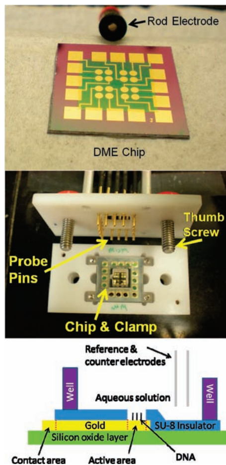
Figure 1. Fabrication of the DME chip. (top) DNA-modified electrode (DME) chip with 16 2 \text{ mm}^2 gold working electrodes shown with a conventional 2 \text{ mm}^2 gold rod electrode. (middle) DME chip in a testing mount with a clamp well that splits the chip into four quadrants of four electrodes. Electrical contact is made to the chip with spring contact probe pins secured into contact with the chip by the thumb screws. (bottom) Side-view illustration of one electrode from the fully assembled DME chip. The working electrode area is defined and separated from the contact area by the SU-8 insulating layer. The solution of interest is confined over the chip by the well, and external reference and counter electrodes complete the circuit.
